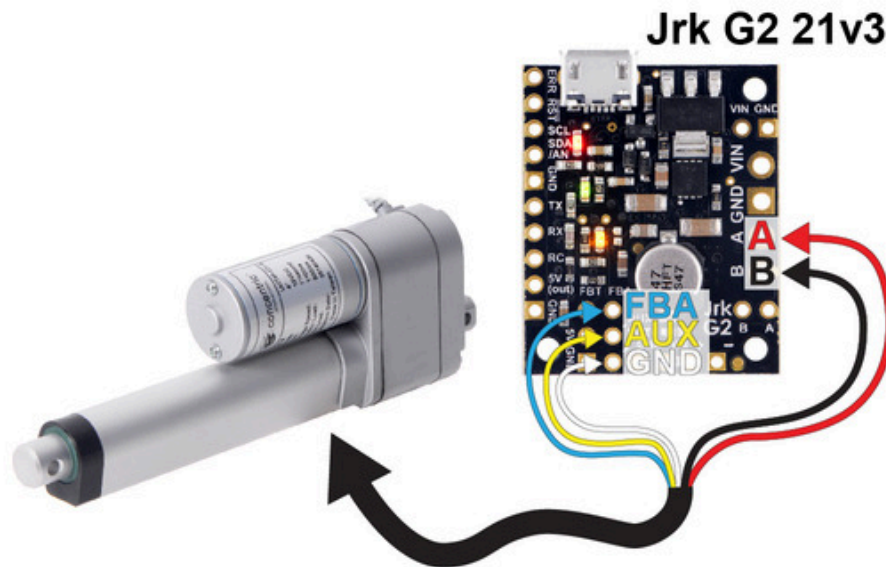
Connecting a light-duty linear actuator with feedback to a Jrk 21v3 motor controller.
