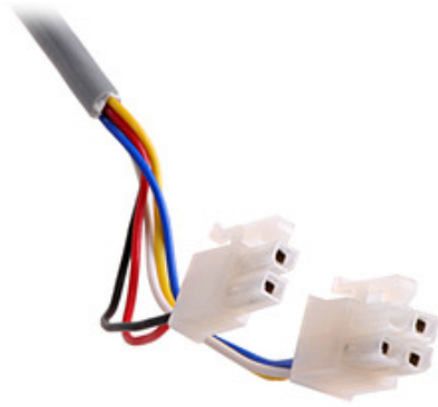
Connectors that terminate the cable ends of Glideforce Light-Duty (LD) linear actuators with feedback.
