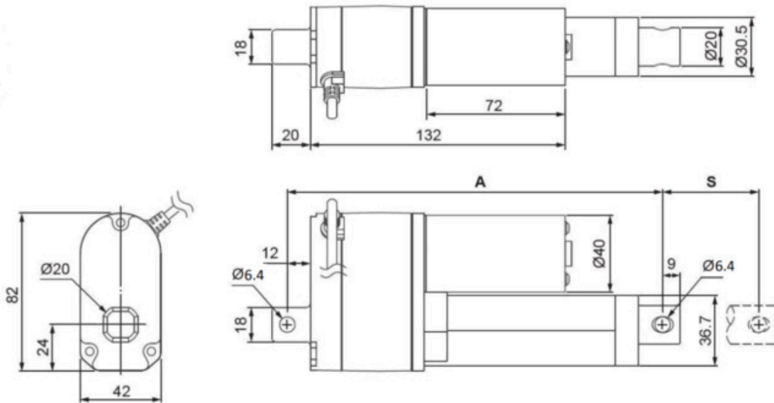
Dimensions of Glideforce LD linear actuators with feedback. Units are mm.
