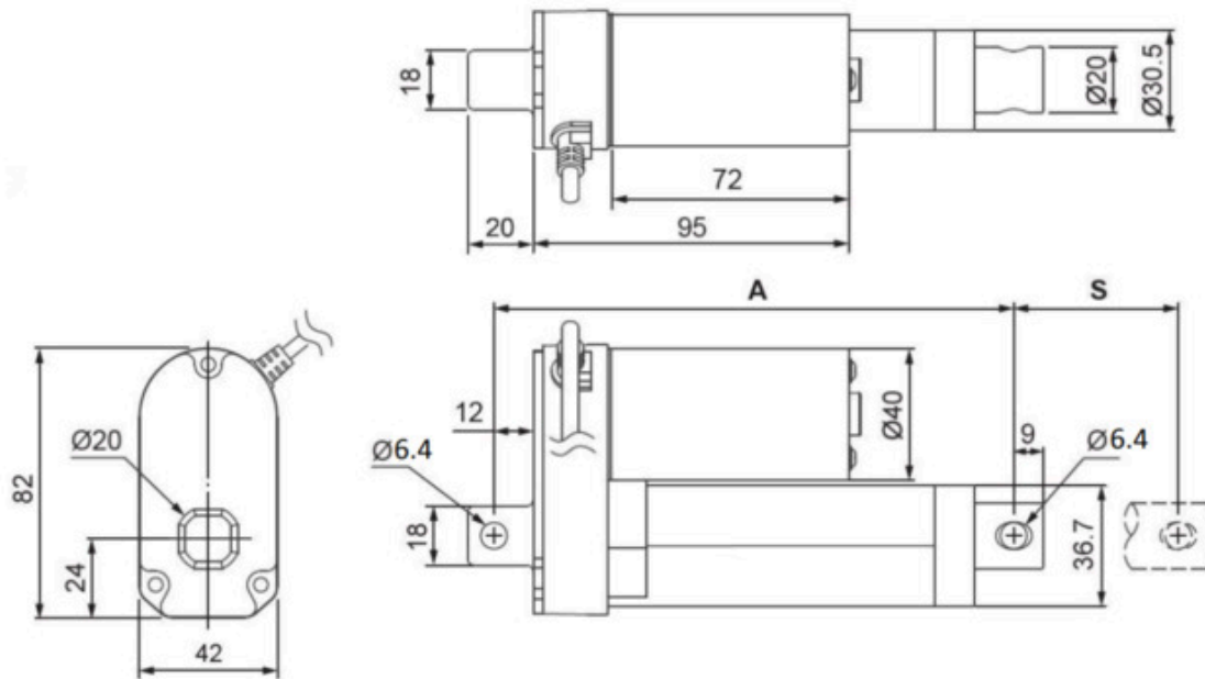
Dimensions of Glideforce LD linear actuators without feedback. Units are mm.
